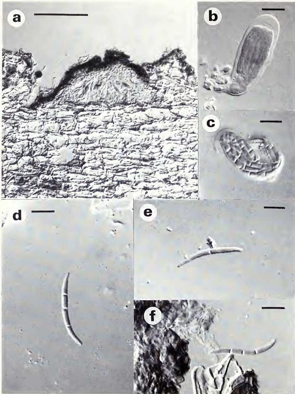
Fig. 18 Leptorhaphis psilotera (Nyl.) Arnold (H-NYL 629) (a) Vertical section of ascoma; scale = 100 \mu\text{m} ; (b), (c) Asci and ascospores; (d), (e), (f) Ascospores; scale = 10 \mu\text{m} .
